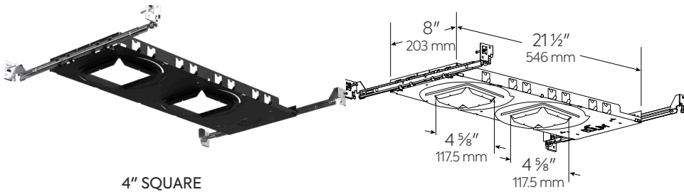
4" SQUARE 45° bidirectional collar rotation for square alignment
