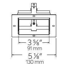
Millwork Adapter (Ordered Separately) Adjusts 1/4" (11mm) - 3/4" (22mm) for wood layer.
