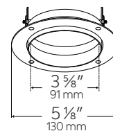
Millwork Adapter (Ordered Separately) Adjusts 1/4" (11mm) - 3/4" (22mm) for wood layer.
