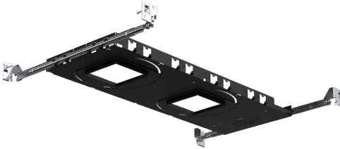
3" SQUARE 45° bidirectional collar rotation for square alignment
