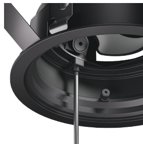
Rotation Lock
