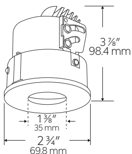
Spackle Frame (Ordered Separately)
