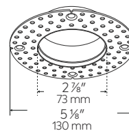
Spackle Frame (Ordered Separately)
