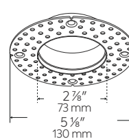
Spackle Frame (Ordered Separately)
