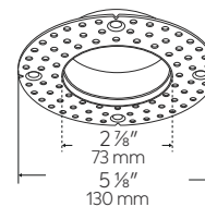
Spackle Frame (Ordered Separately)
