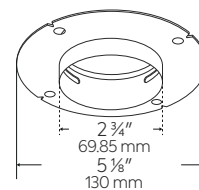
Millwork Adapter (Ordered Separately) Adjusts 3/4" (11mm) - 3/4" (22mm) for wood layer.
