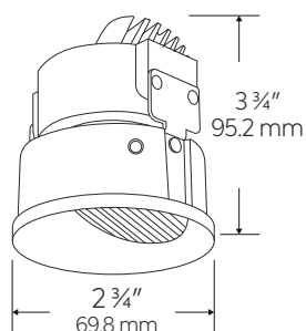
Spackle Frame (Ordered Separately)
