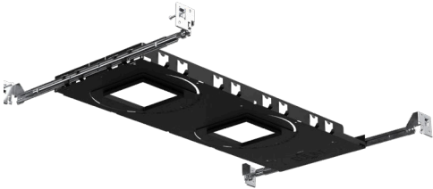
2" SQUARE 45° bidirectional collar rotation for square alignment
